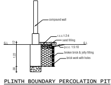
PLINTH BOUNDARY PERCOLATION PIT
