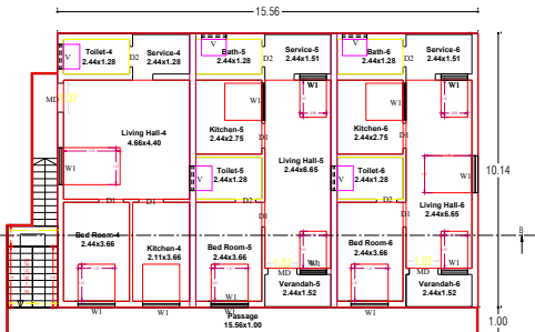
PRO.FIRST FLOOR PLAN
