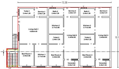
EX.GROUND FLOOR PLAN
