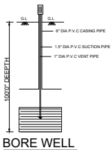
BORE WELL
