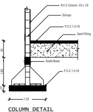
COLUMN DETAIL
