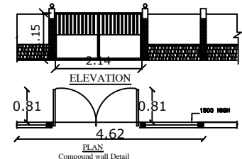
Compound wall Detail
