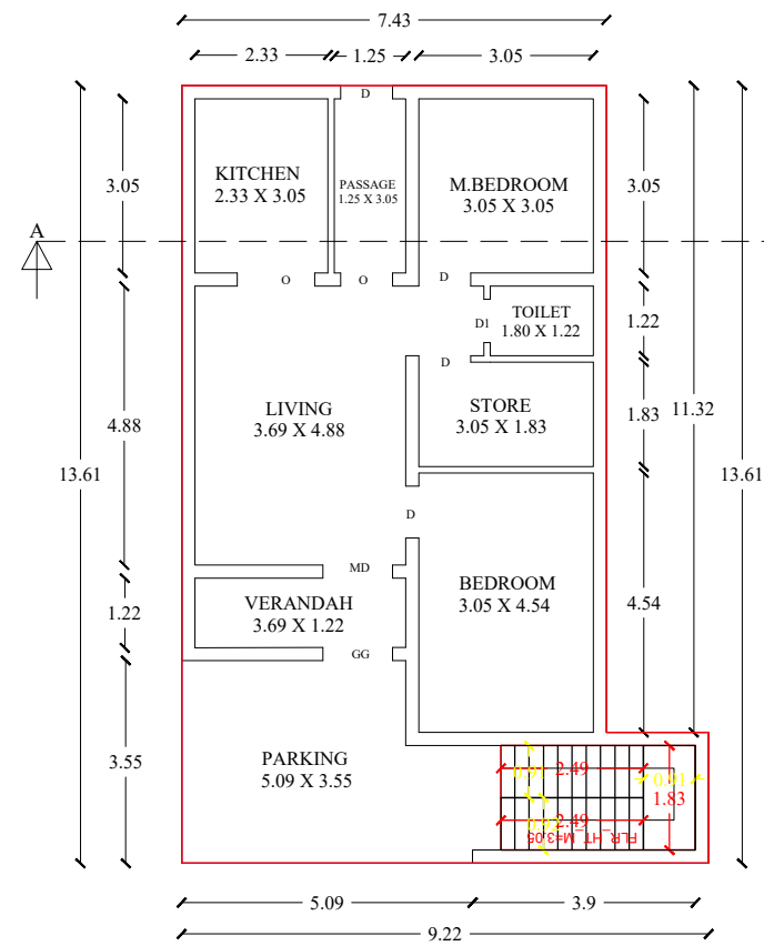
EXI.GROUND FLOOR PLAN
