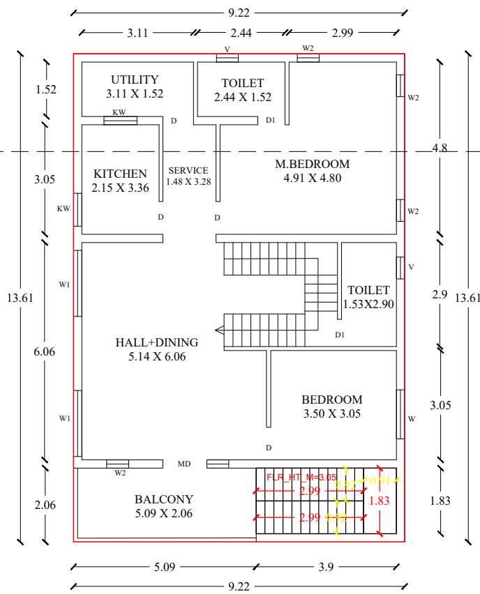
EXI.FIRST FLOOR PLAN
