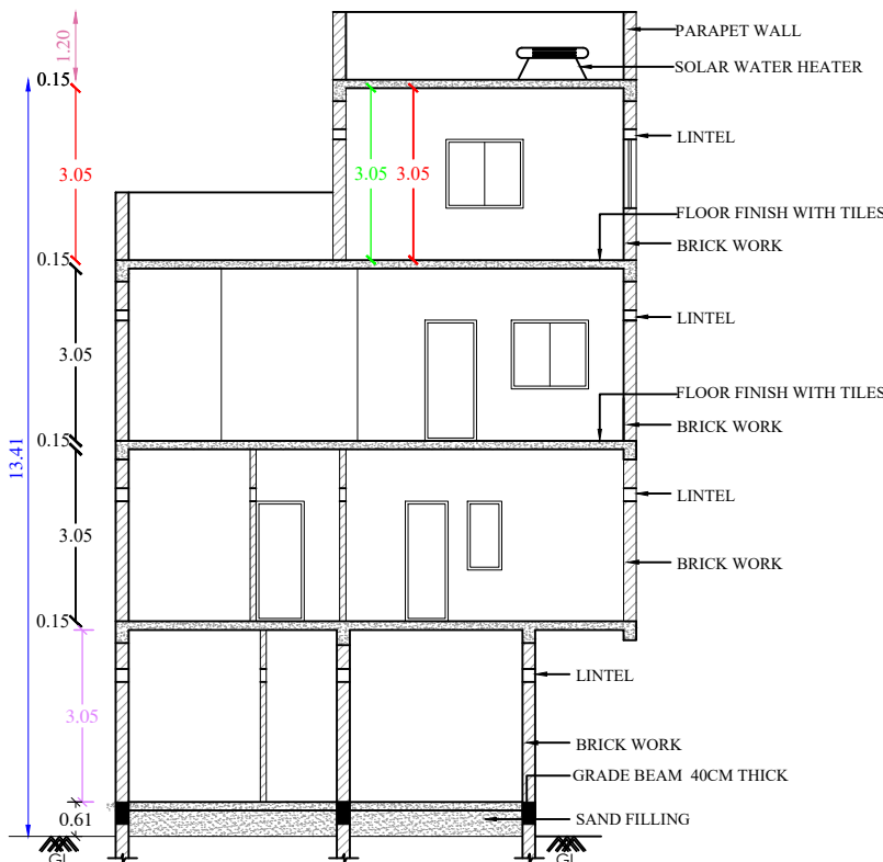
SECTION -AA1
