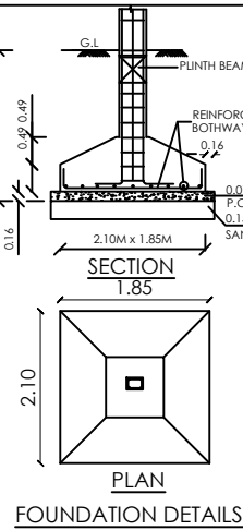
FOUNDATION DETAILS
