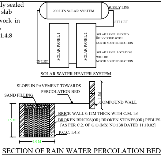
SECTION OF RAIN WATER PERCOLATION BED
