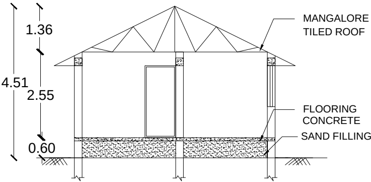
SECTION ON BR
