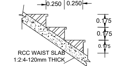
STAIR CASE STEPS SCALE 1:25
