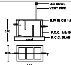
Septic tank detail
