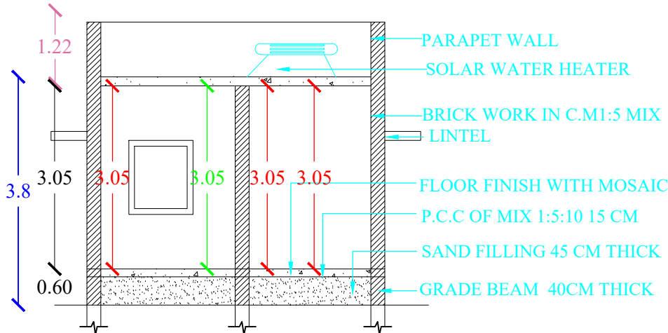
SECTION- AA1
