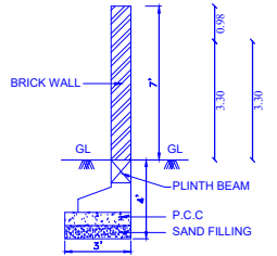
COMPOUND WALL DETAIL
