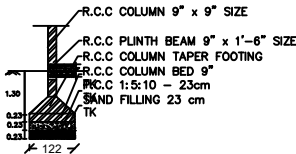
SECTION
