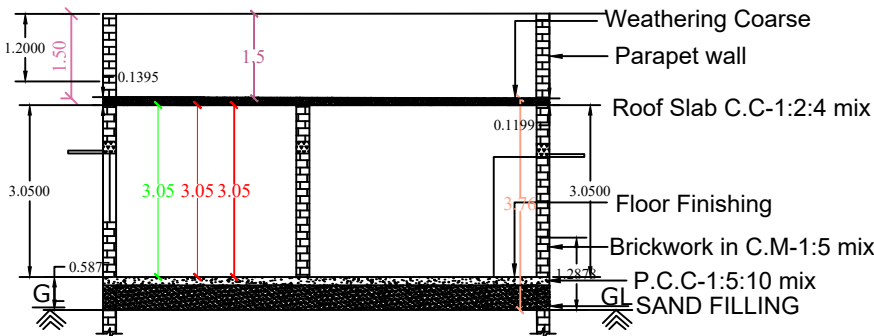
CROSS SECTION ON XX
