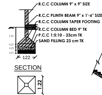
COLUMN DETAILS PLAN
