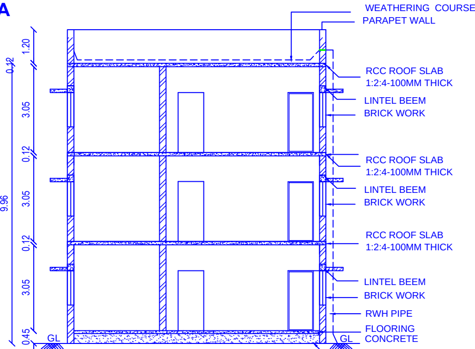
SECTION - XY
