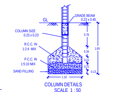
COLUMN DETAILS
