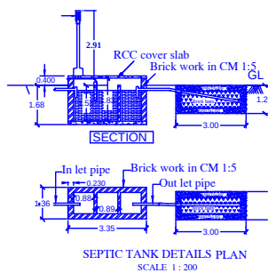
SEPTIC TANK DETAILS PLAN
