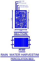
RAIN WATER HARVESTING PERCOLATION BED
