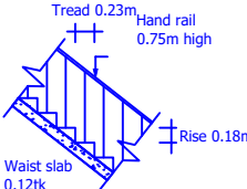
STAIR DETAILS
