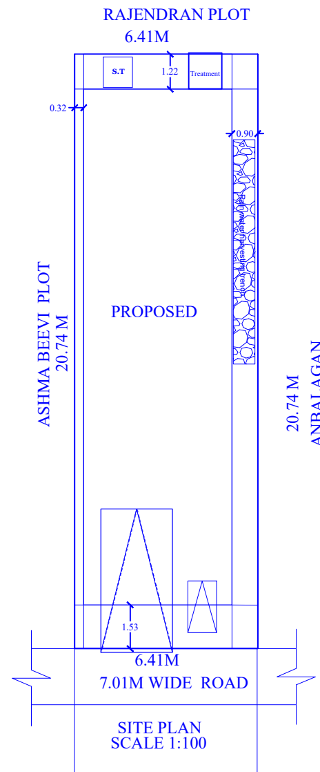
NOTE 1. Certified That Rain Water Harvesting And Waste Water Recycling Systems Shall Be Provided As per Building Rule no: 17A 2. Solar water Heater System provided at the Topmost Level of the building 3. Map is Oriented To Magnetic North 4. All Dimensions Are In Metre 5. Sewage line should be connected in the exiads
