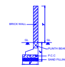
FOUNDATION DETAILS Scale 1:50
