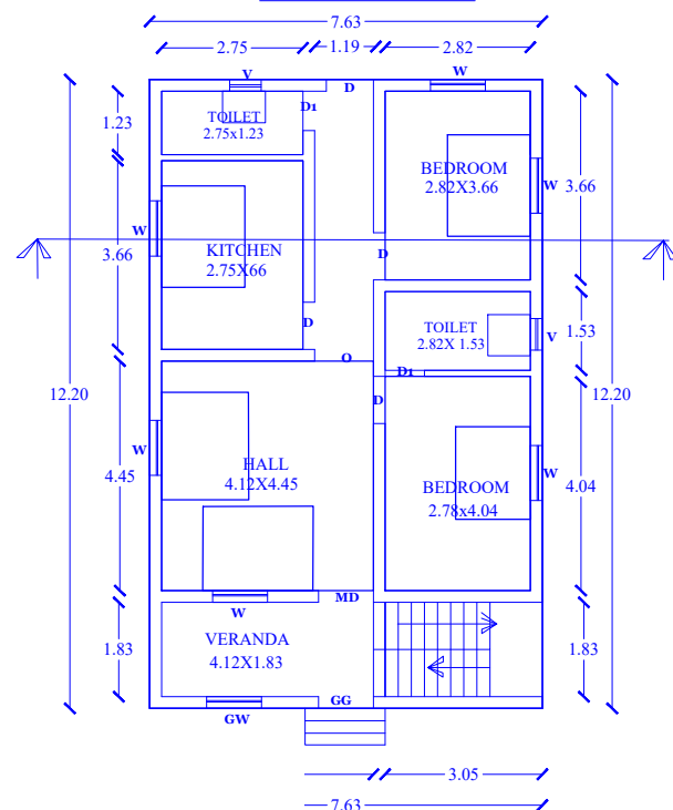
D FLOOR PLAN
