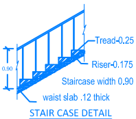
STAIR CASE DETAIL
