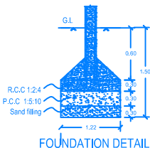
FOUNDATION DETAIL
