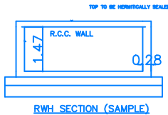
RWH_SECTION (SAMPLE)
