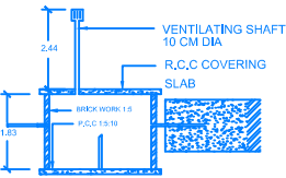
SEPTIC TANK DETAIL
