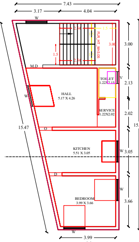
SECOND FLOOR PLAN (Residential)
