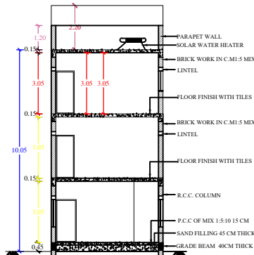
SECTION-AA1
