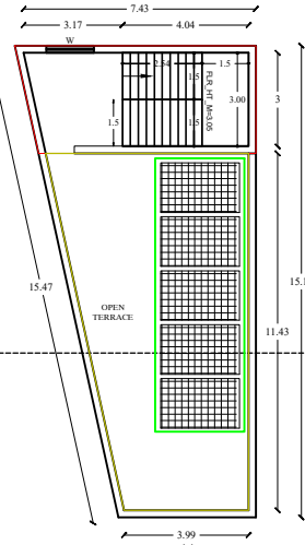
TERRACE FLOOR PLAN
