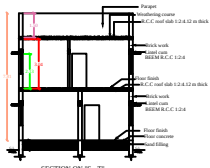
SECTION ON 'X-X'
