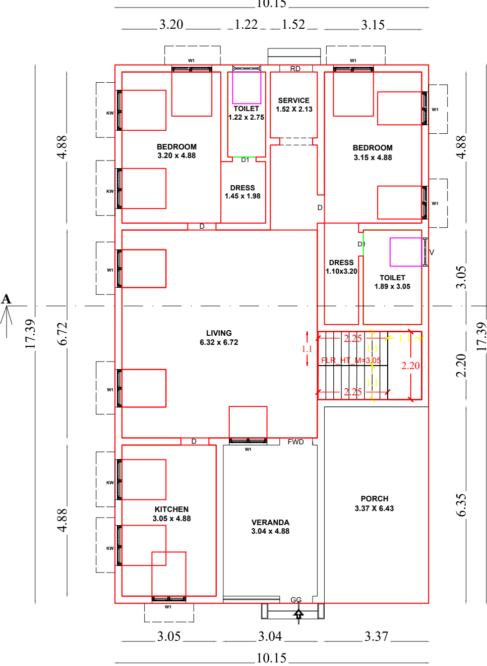
FLOOR PLAN
