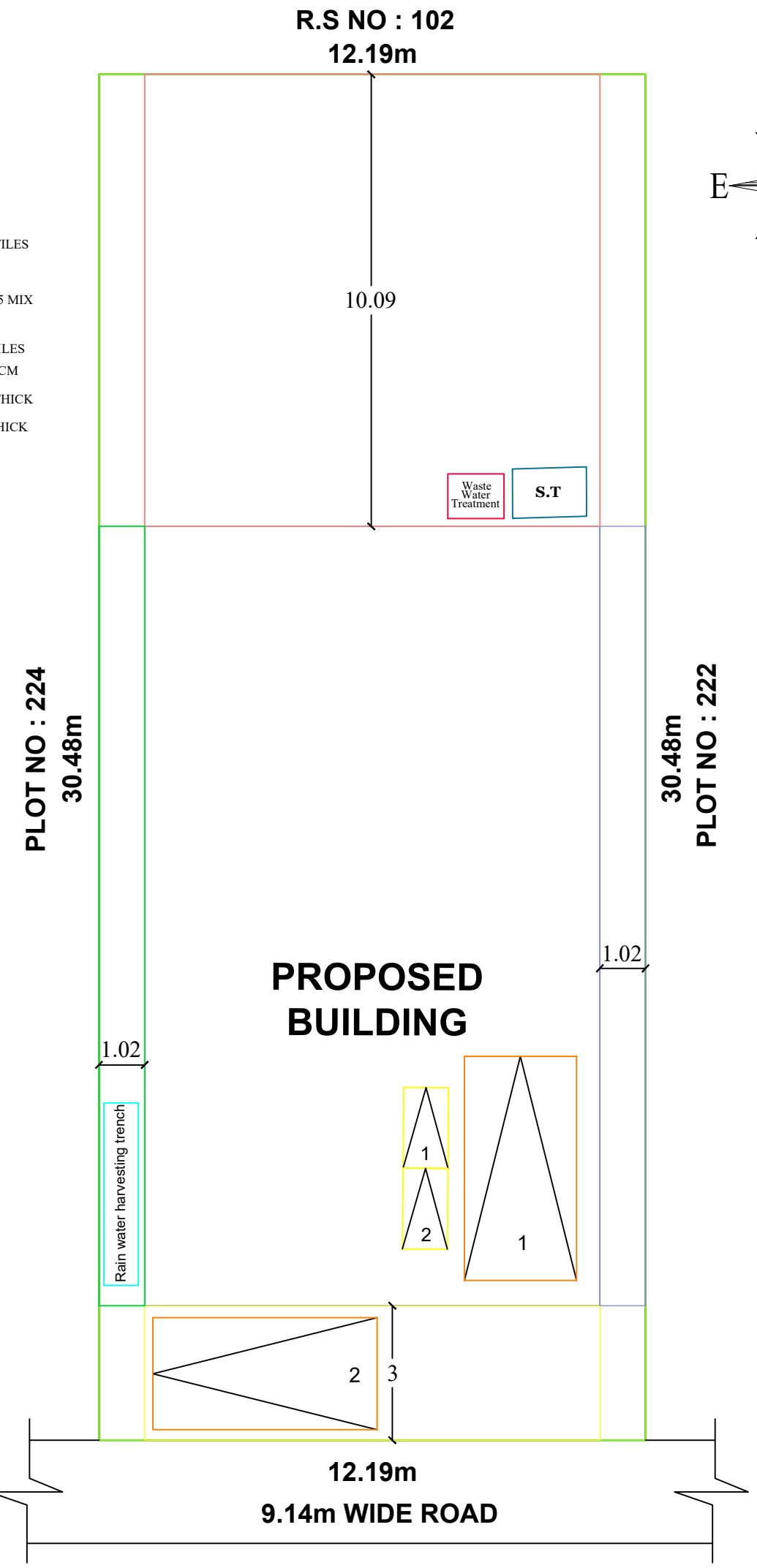
SITE PLAN
