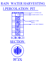
RAIN WATER HARVESTING PLAN
