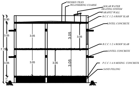
SECTION ON-AA'
