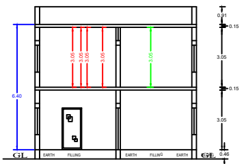
SECTION "A-B"
