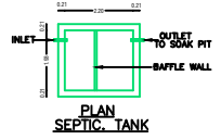
PLAN SEPTIC TANK
