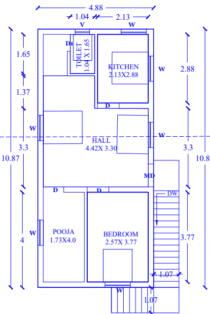
PRO. FLOOR PLAN
