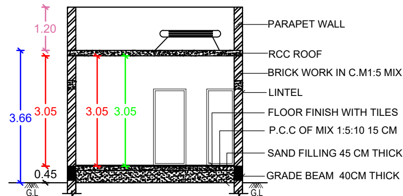
SECTION-AA1
