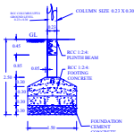
FOUNDATION DETAILS Scale 1:30
