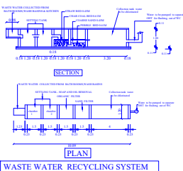
WASTE WATER RECYCLING SYSTEM
