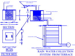
PLAN FILTER BED
