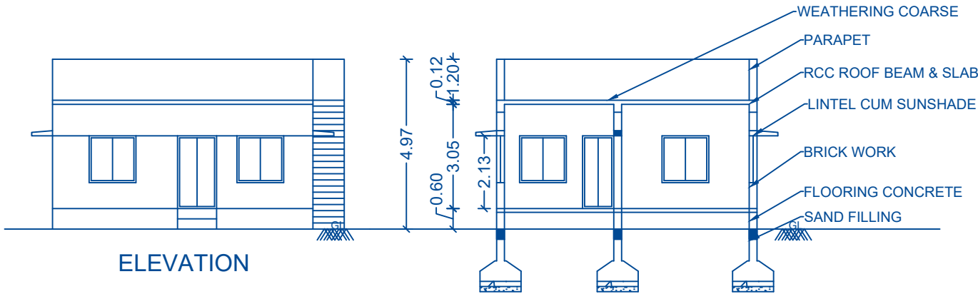
SECTION ON "X-Y"
