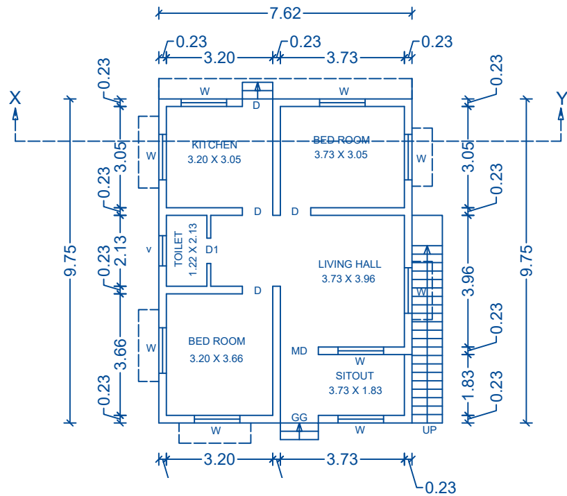
FLOOR PLAN
