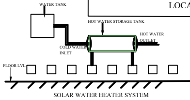
SOLAR WATER HEATER SYSTEM
