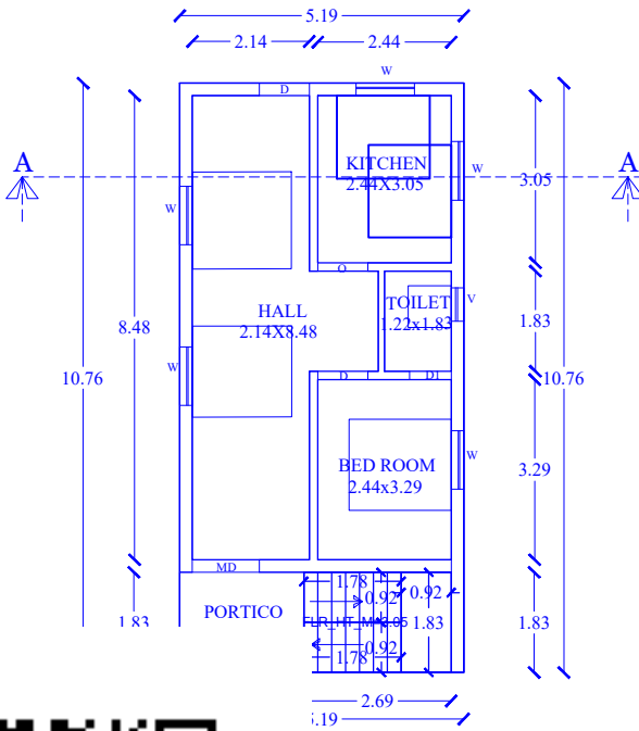
FLOOR PLAN
