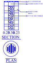
RAIN WATER HARVESTING PERCOLATION PIT
