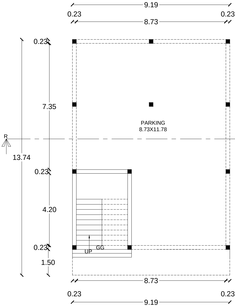
PRO - STILT FLOOR PLAN
