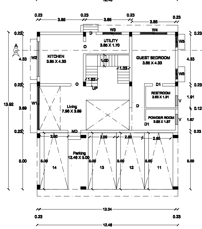
GROUND FLOOR PLAN BLOCK.2
