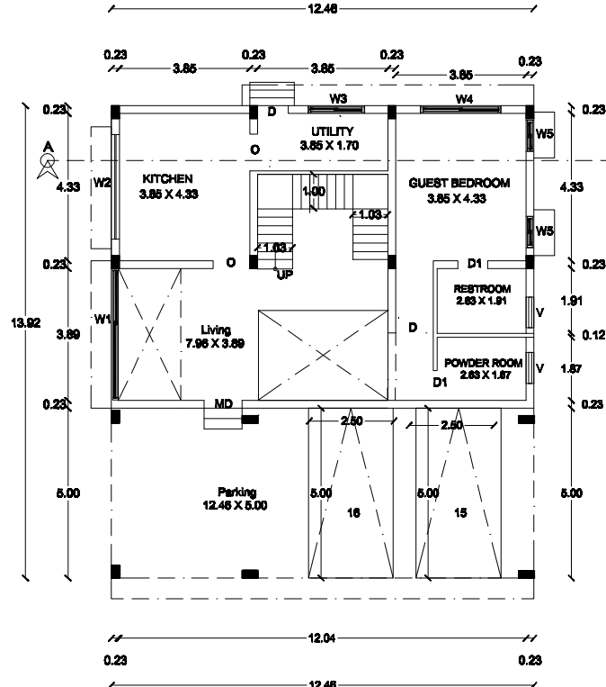
GROUND FLOOR PLAN BLOCK.3
