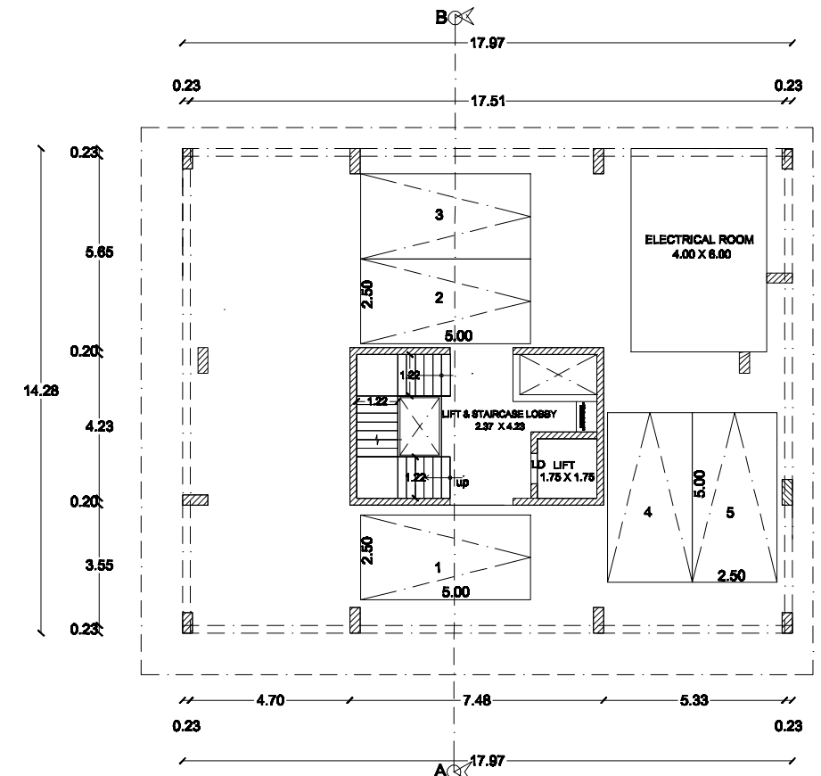
STILT FLOOR PLAN BLOCK - 1
