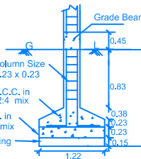
COLUMN DETAILS NOT TO SCALE
