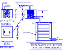
RAIN WATER COLLECTION SYSTEM FROM TERRACE
