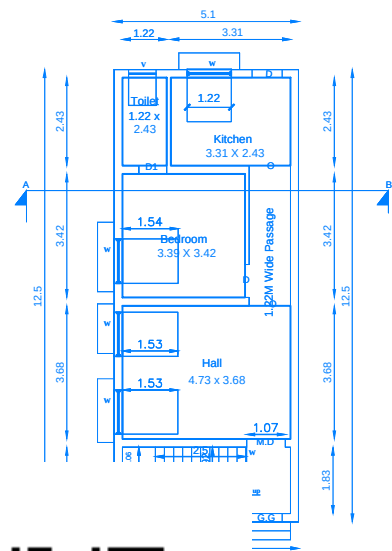
FLOOR PLAN
