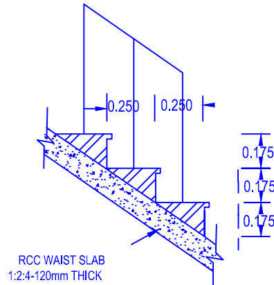
STAIR CASE DETAILS NOT TO SCALE
