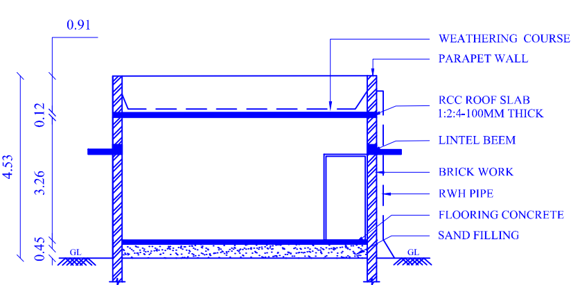
SECTION -XY
