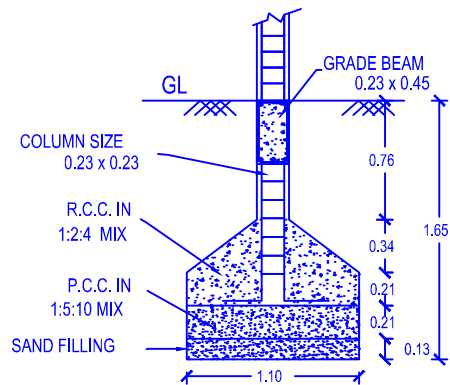
COLUMN DETAILS SCALE 1 : 50
