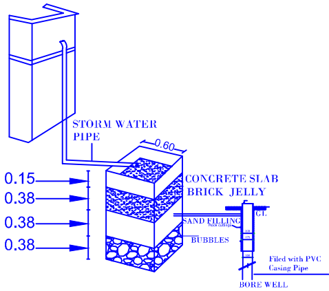
FILTER TANK RAIN WATER HARVESTING
