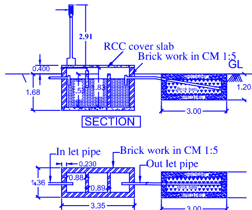
SEPTIC TANK DETAILS PLAN SCALE 1 : 200
