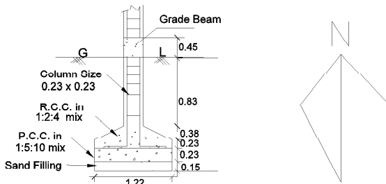
COLUMN DETAILS NOT TO SCALE
