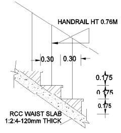
STAIR CASE STEPS SCALE 1:25
