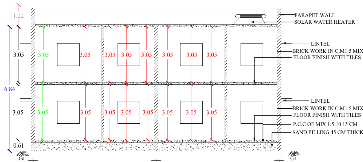
SECTION ON A-A1
