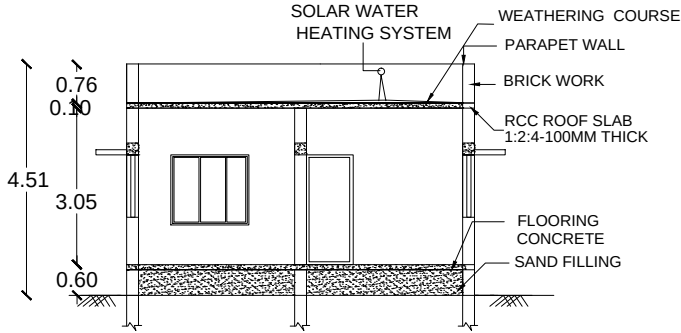
SECTION ON BR
