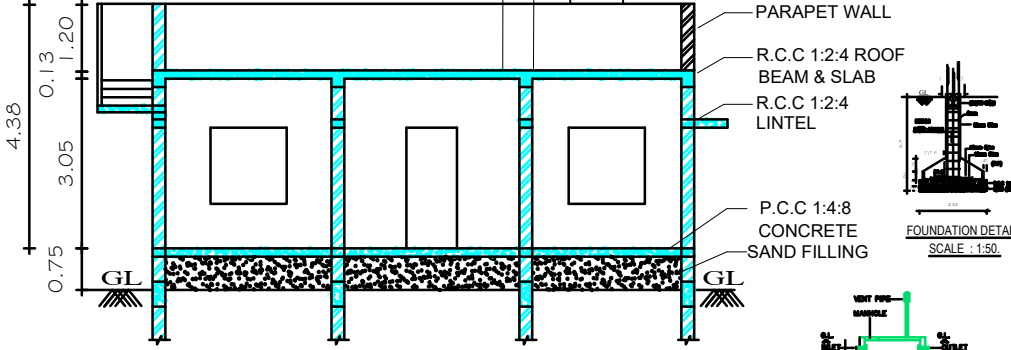
SECTION "A-B"
