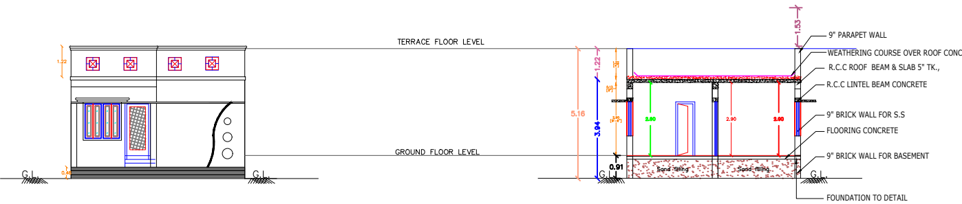
FRONT ELEVATION
