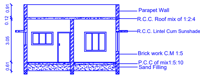
SECTION ON RS
