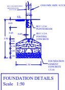
FOUNDATION DETAILS Scale 1:50
