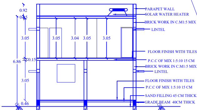
SECTION ON A-A1
