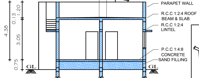
SECTION "A-B"
