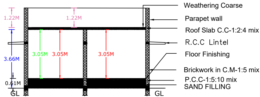
SECTION ON XX
