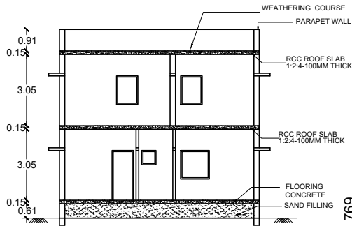
SECTION NP
