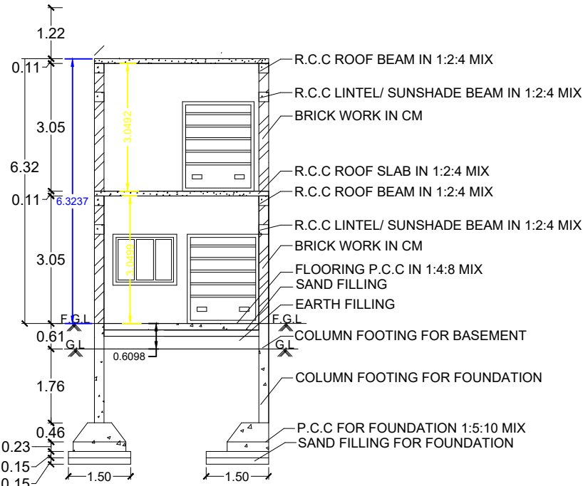
SECTION ON-AA
