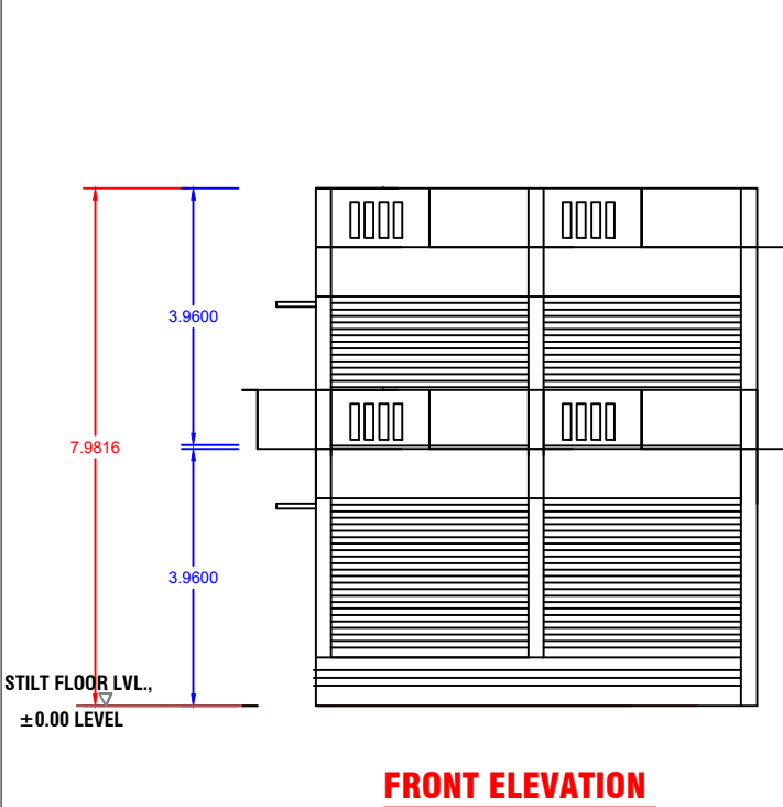
FRONT ELEVATION
