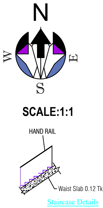
Staircase Details
