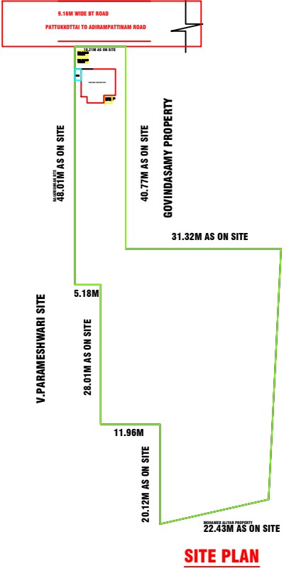
SITE PLAN
