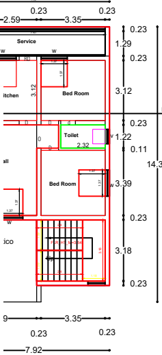
O. FIRST FLOOR
