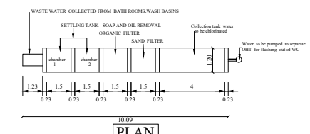
WASTE WATER RECYCLING SYSTEM
