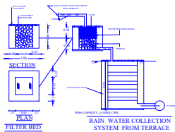
RAIN WATER COLLECTION SYSTEM FROM TERRACE
