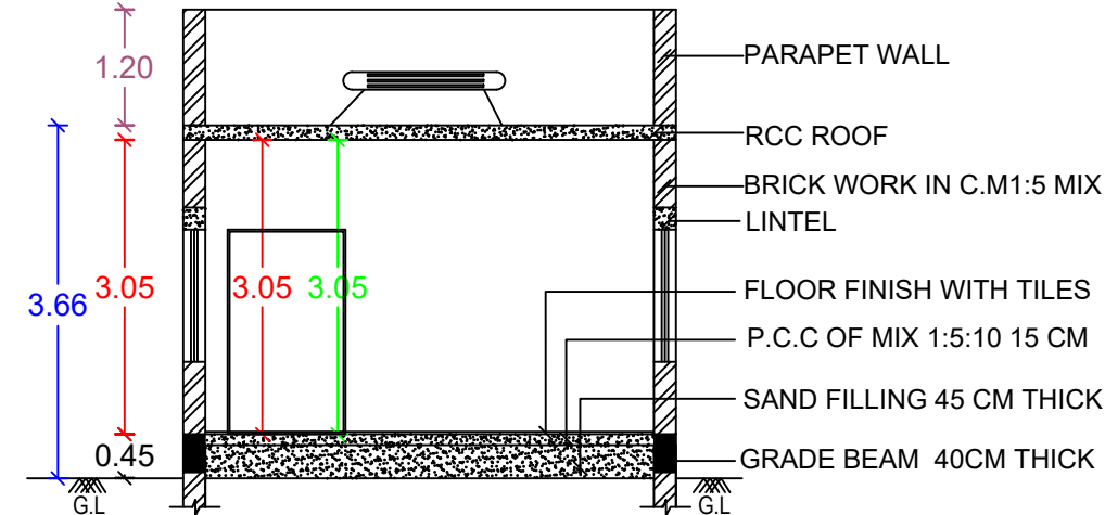
SECTION-AA1
